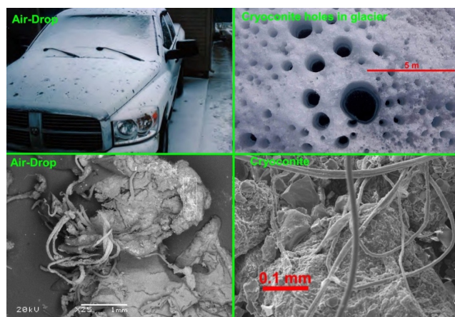
Figure 4: Upper Left: Air-Drop Distribution; Upper Right: Cryoconite-hole Distribution in Glacier; Lower Left: Air-Drop Synthetic or Proto-Cryoconite; Lower Right: Natural Cryoconite.
